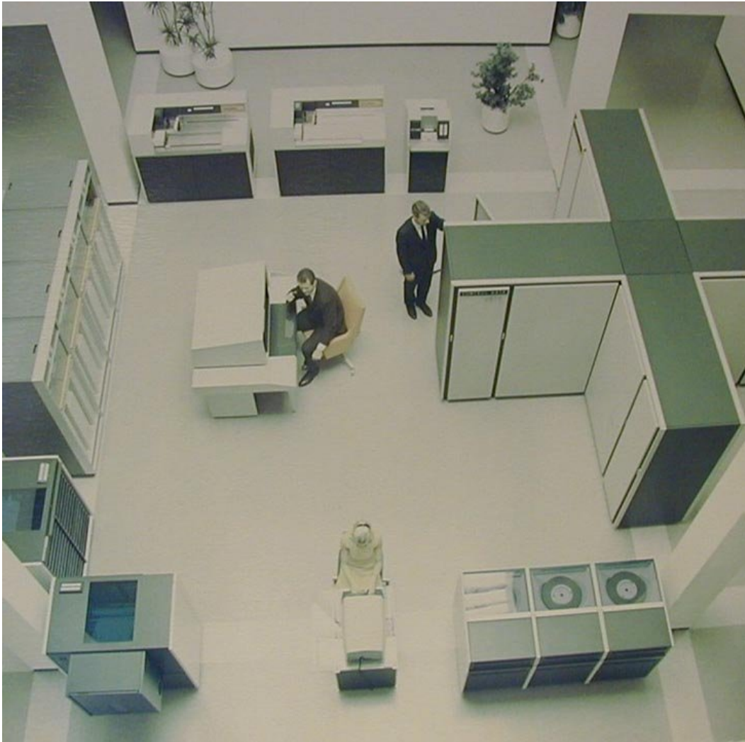
CDC 6600 1Mflops
