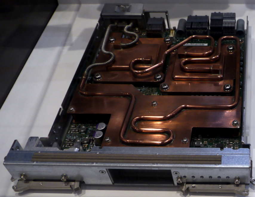
Post-K Computer Prototype CPU Memory Unit
